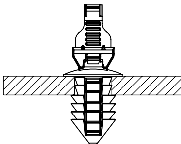
ASSEMBLED VIEW
